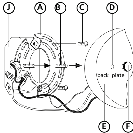
Drawing 2 - Final Assembly
